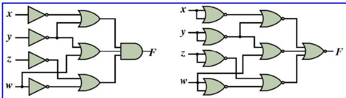
OR-AND
