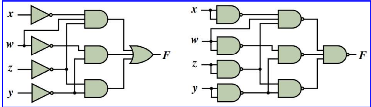
AND-OR
